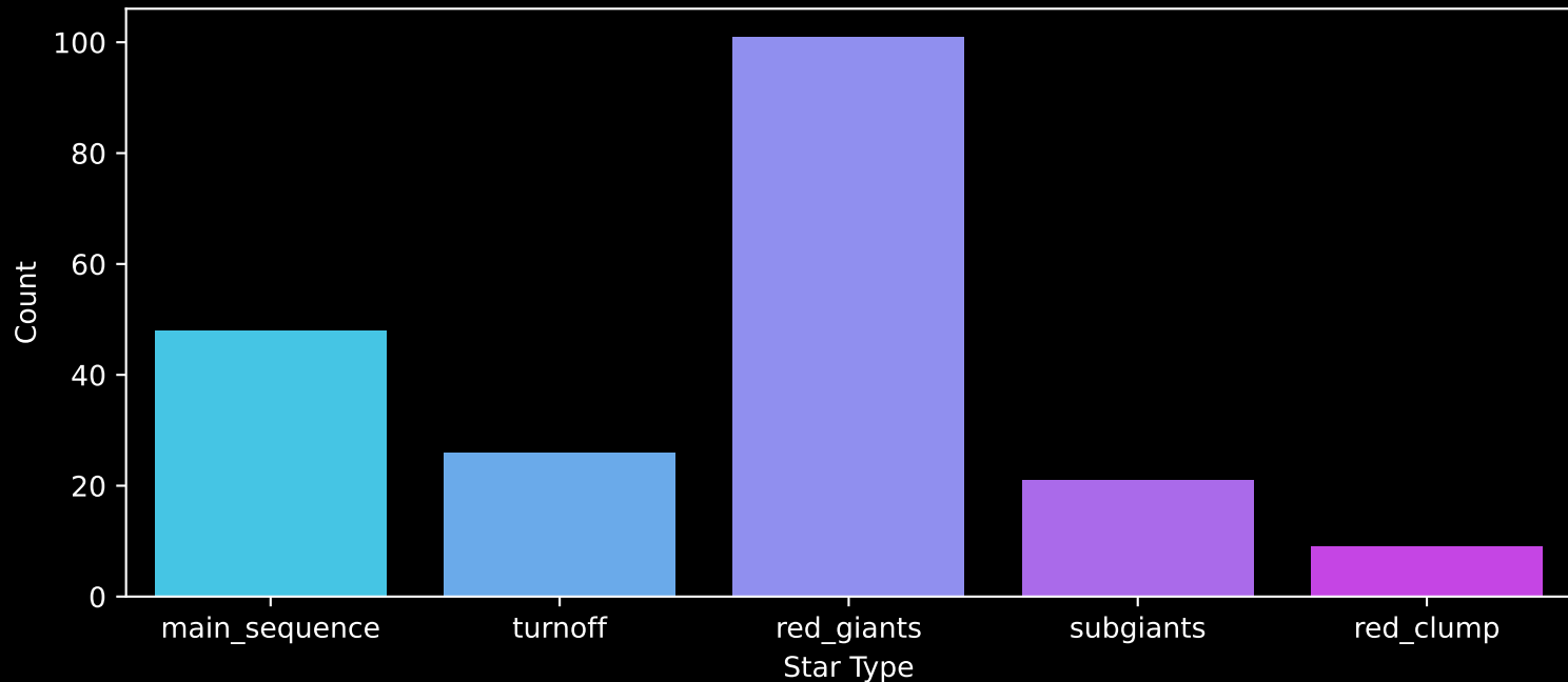
APOGEE DR17 Field: [N5634SGR2-RV_btx] Count plot of Star Type
