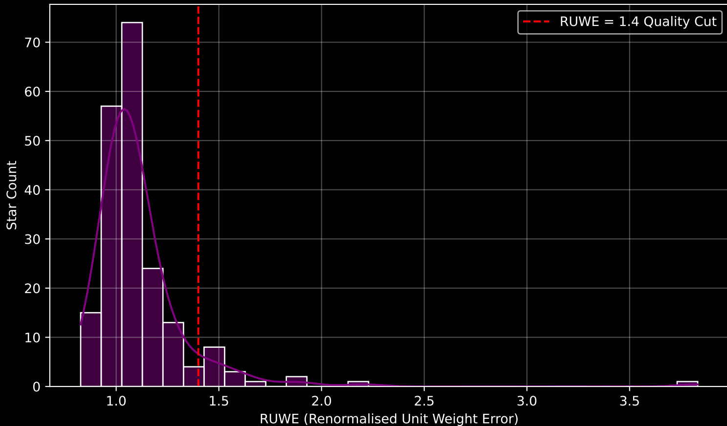
GAPOGEE DR17 Field [N5634SGR2-RV_btx] RUWE Distribution (n= 203)
