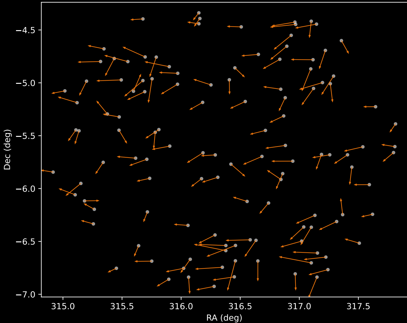
APOGEE DR17 Cluster 2 Proper Motion Vectors (n=121)
