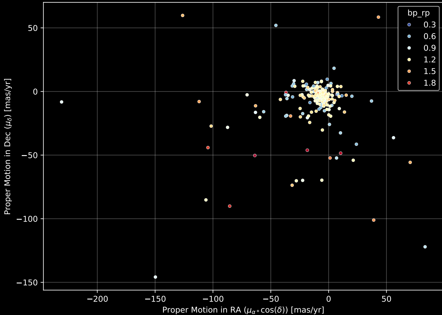
APOGEE DR17 Field: [N5634SGR2-RV_btx] Proper Motion Diagram (n= 205)
