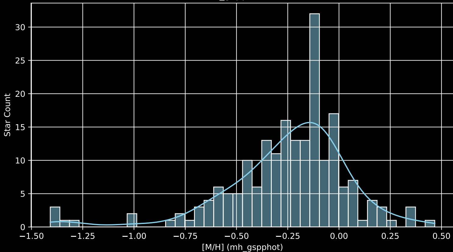
APOGEE DR17 Field: [N5634SGR2-RV_btx [M/H] (mh_gspphot) (n= 201)
