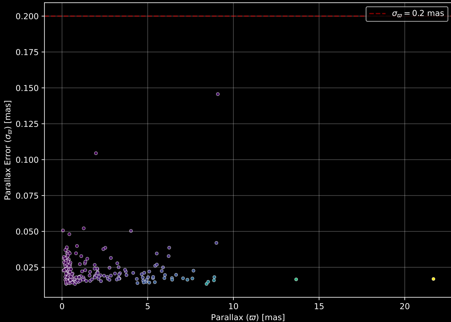
APOGEE DR17 Field: [N5634SGR2-RV_btx] Parallax Quality (n= 205)
