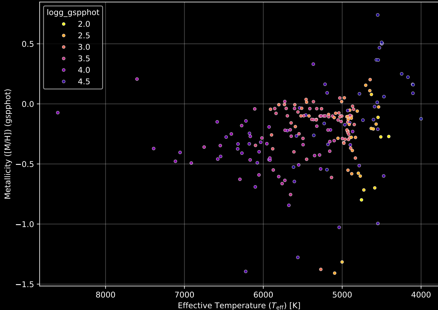
APOGEE DR17 Field: [N5634SGR2-RV_btx] Stellar Population Parameters (n= 205)
