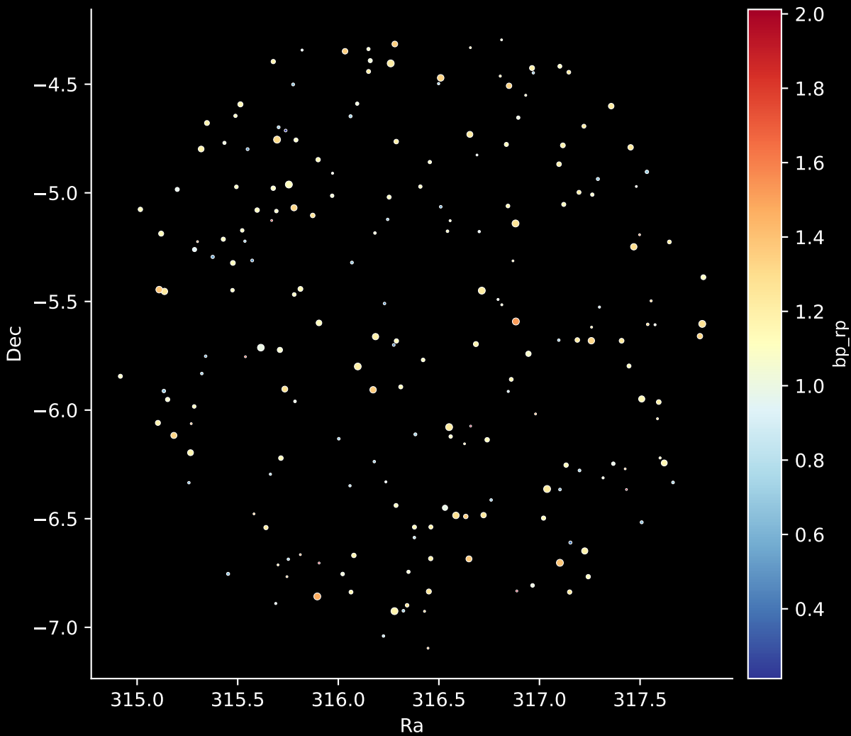
APOGEE DR17 Field: [N5634SGR2-RV_btx] Stars: 205
